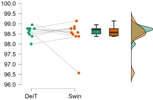
DeiT - Swin
