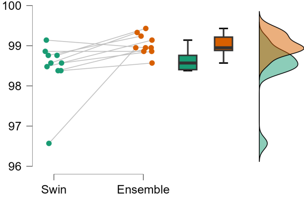
Swin - Ensemble
