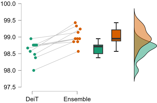
DeiT - Ensemble
